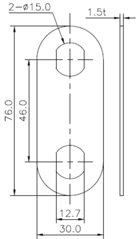
BACK PLATE
