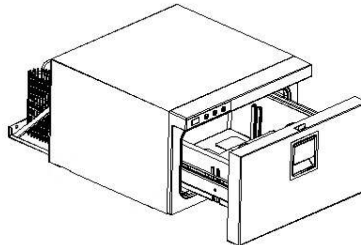
Three-Dimension View of Drawer 16
