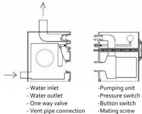
*Illustration Diagram representing the split system
